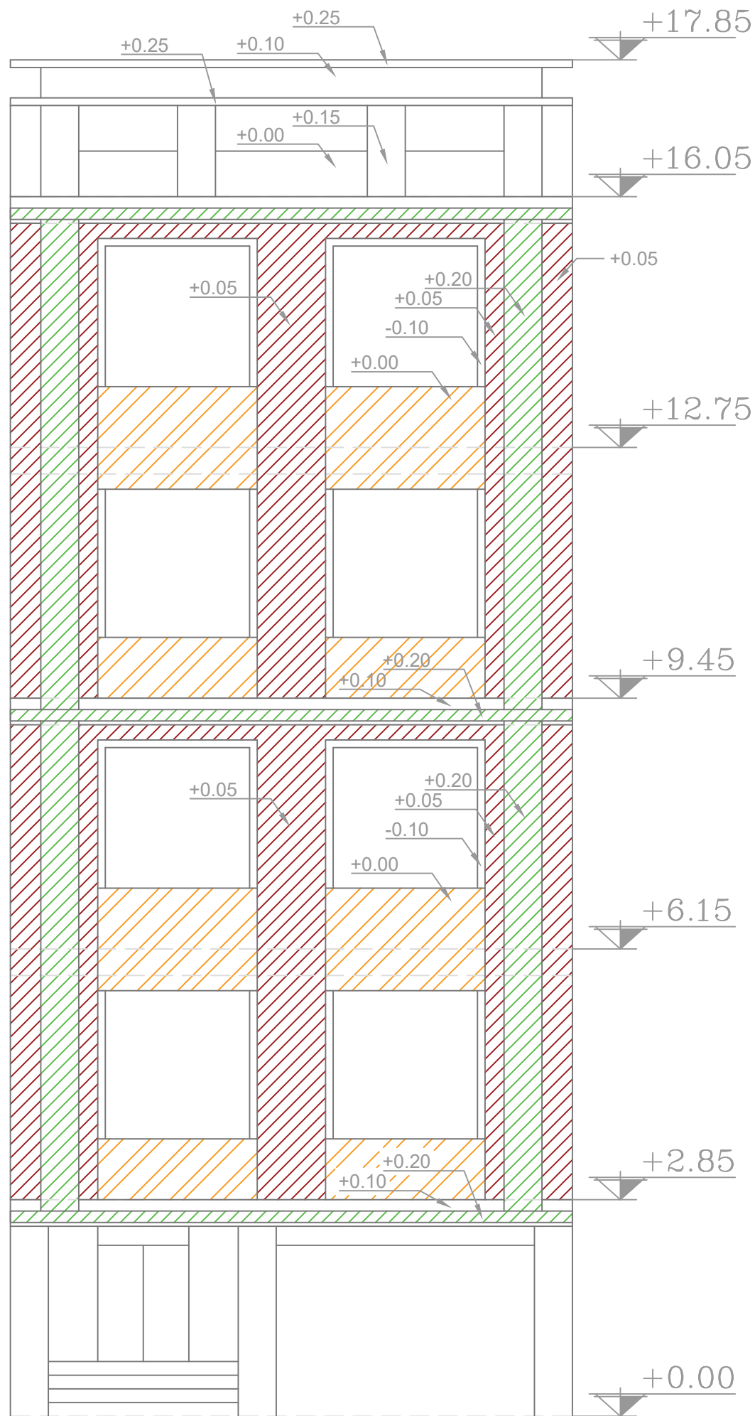
NORTH FACADE / HEIGHT CODE
