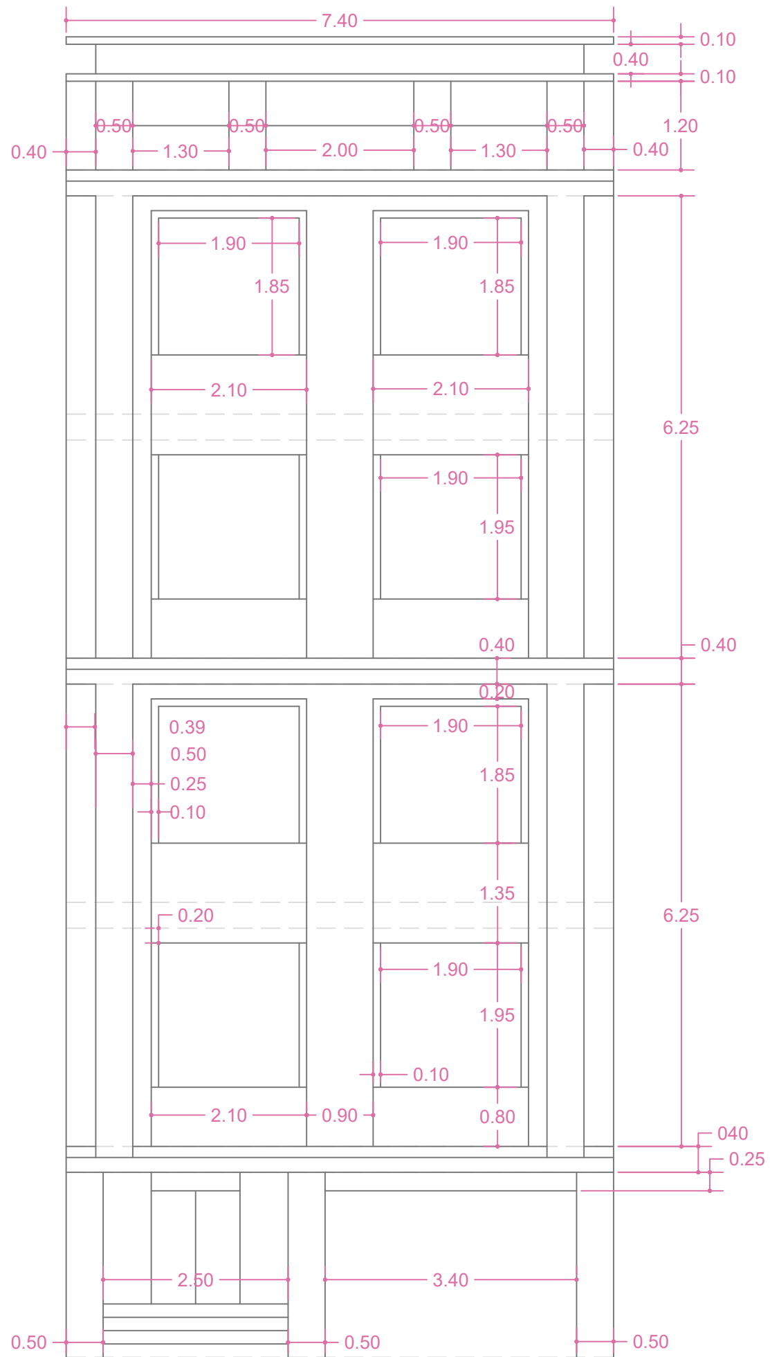
NORTH FACADE / DIMENSIONS
